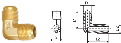
二通弯头(同径) Union Elbow Straight
